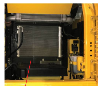
Debris Screen
