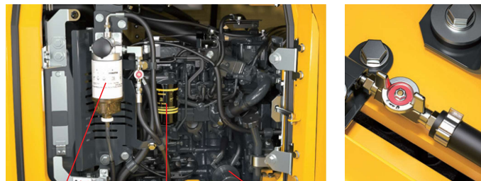
Fuel pre-filter (With water separator)
