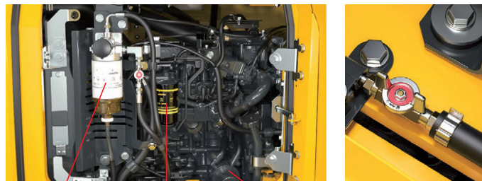
Fuel pre-filter (With water separator)
