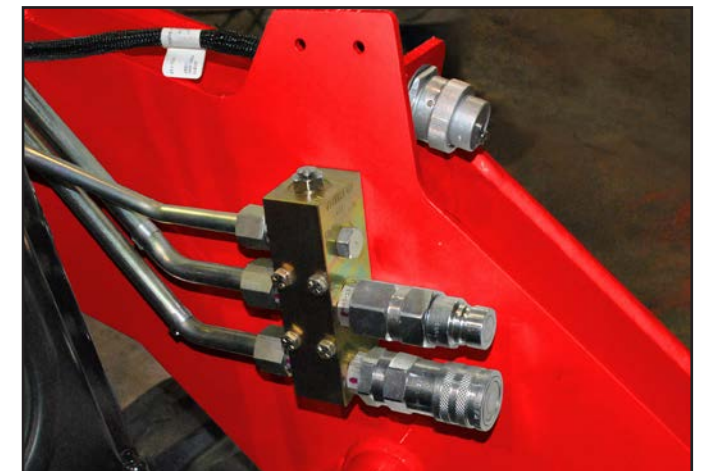
Pressure relieving attachment couplers and an available attachment control kit make Takeuchi skid steers very versatile.
